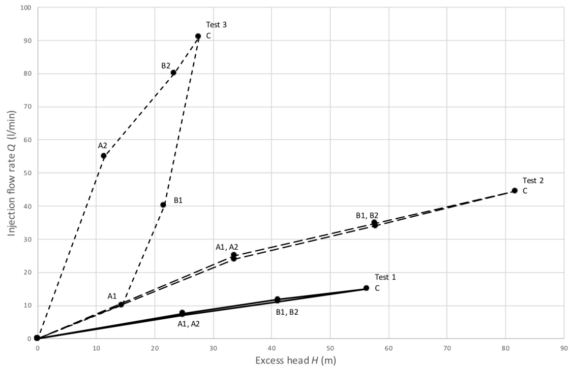
Fig. 5: Example plots of packer test analysis ( data from Table 3 )
