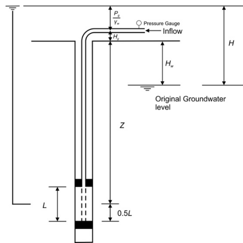
(b) pressure gauge in the above ground injection pipework (double packer test shown)
