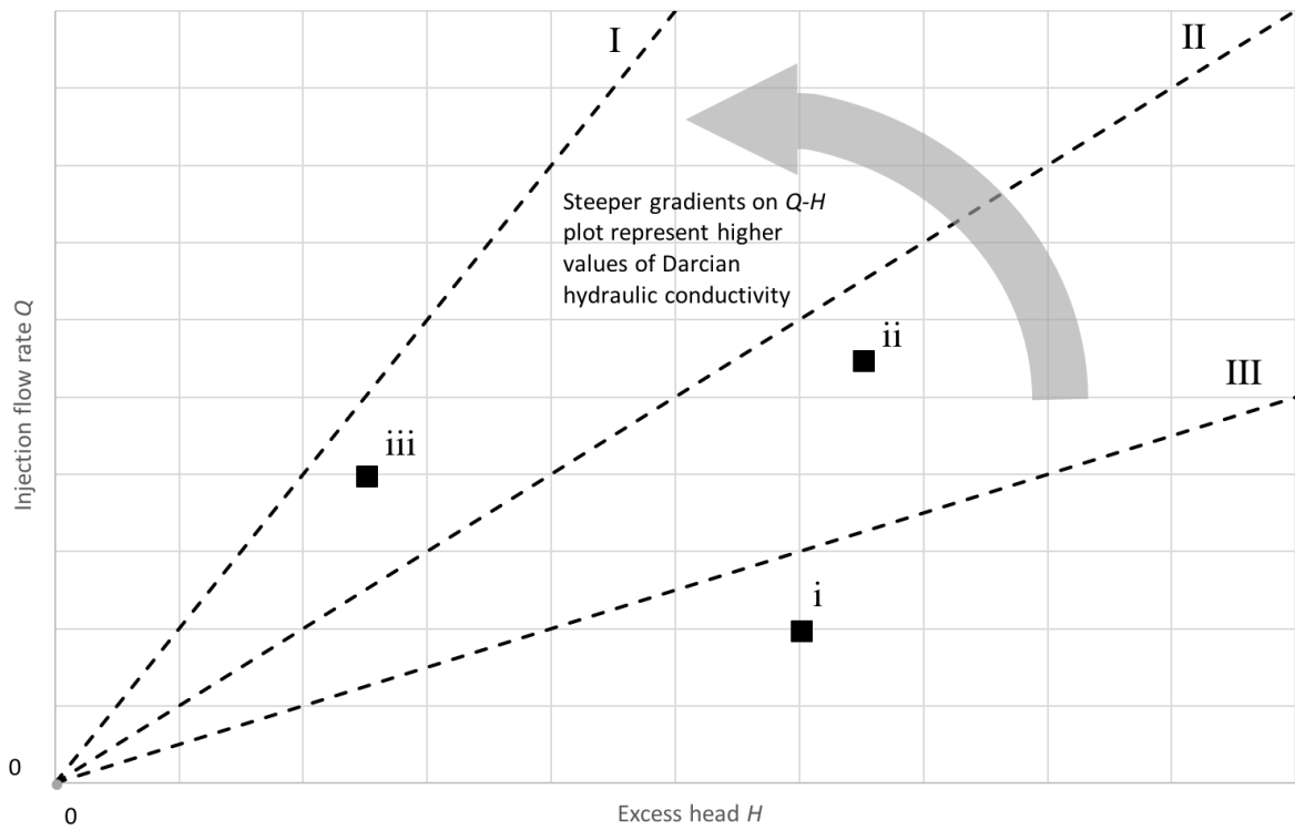
Fig. 2: Example plot of injection flow rate Q vs. applied excess head H
