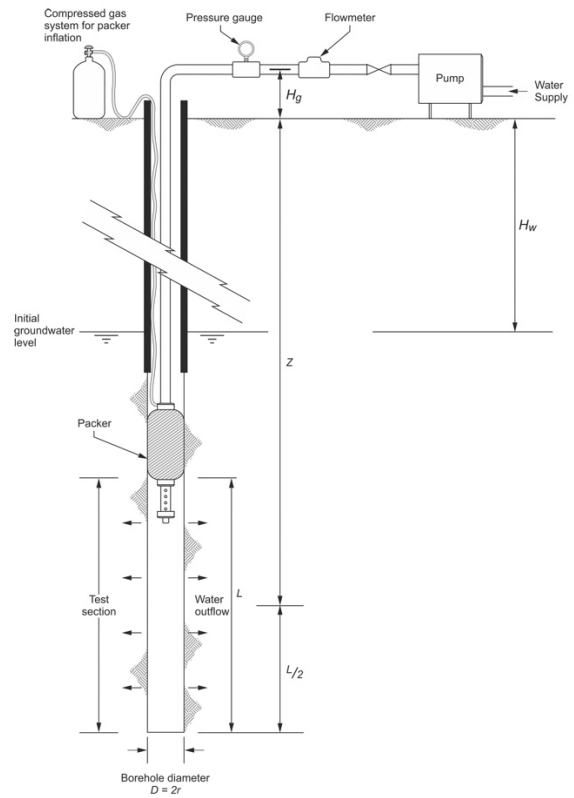
(b) Single packer test
