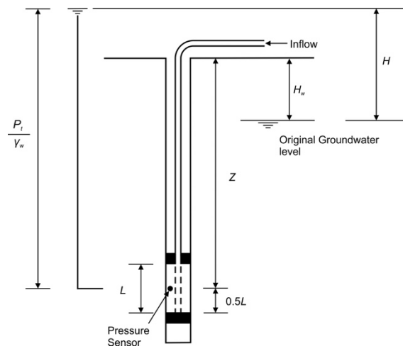
(a) pressure transducer within the test section (double packer test shown)
