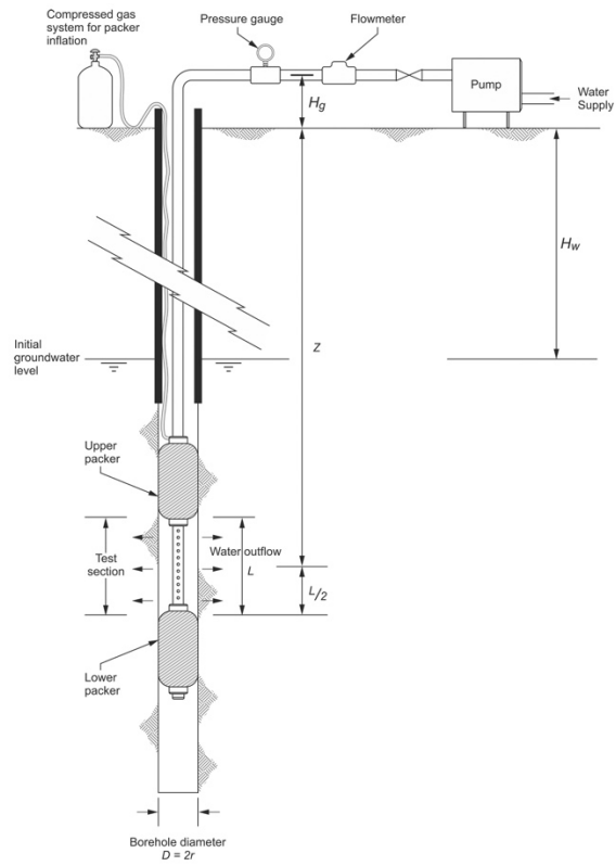
(a) Double packer test
